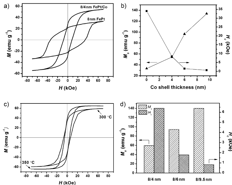
Figure 3. a) Room-temperature hysteresis loops of fct-FePt NPs and 8/4 nm FePt/Co core/shell NPs. b) Co shell-thickness-dependent M_s and H_c for the FePt/Co core/shell NPs. c) Room-temperature hysteresis loops of the FePt/Co nanocomposites annealed from 8/4 nm FePt/Co core/shell NPs at 300 and 350 °C. d) M_s and H_c of the FePt/Co nanocomposites annealed from FePt/Co core/shell NPs with different Co shell thickness.
